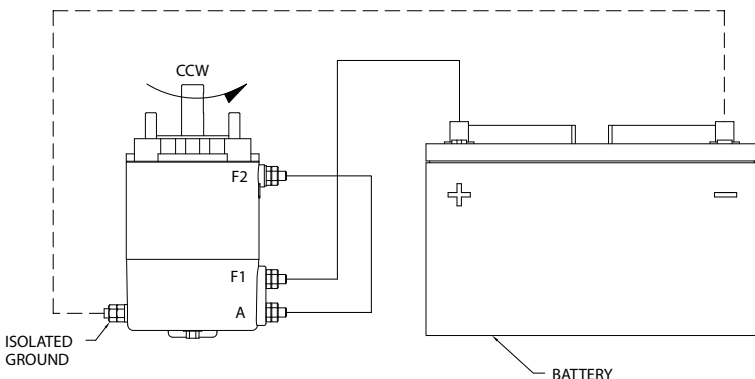
FIGURE-2 MOTOR-COUNTER CLOCKWISE ROTATION
