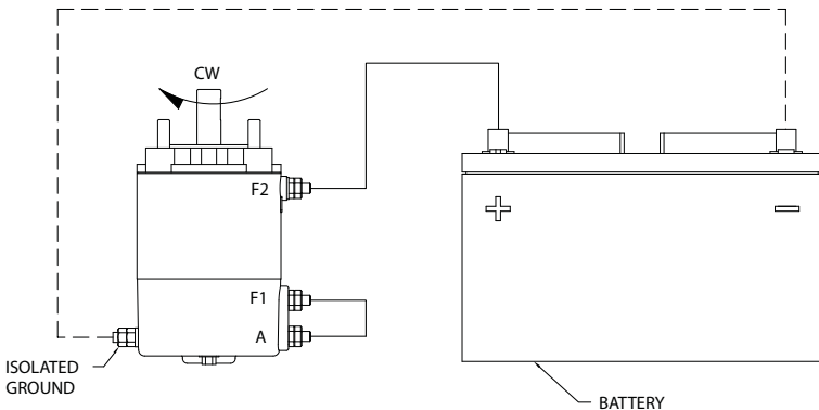
FIGURE-1 MOTOR-CLOCKWISE ROTATION
