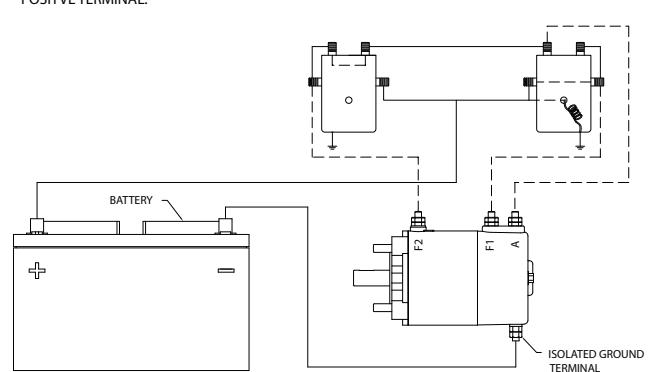
SOLENOIDS TO MOTOR CONNECTIONS
