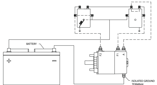
SOLENOIDS TO MOTOR CONNECTIONS
