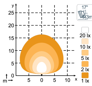
N4403 QD, N4404, 2500lm Diffused
